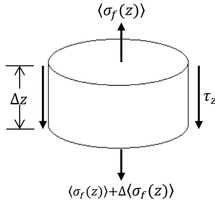
Figure 3. Free body diagram of an increment of fiber embedded in a matrix
